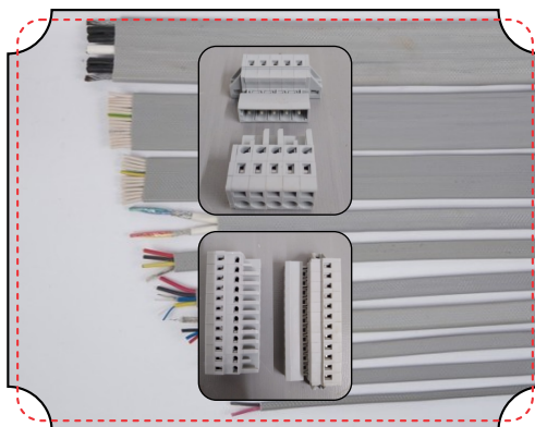
Plugable Traveling Cable
